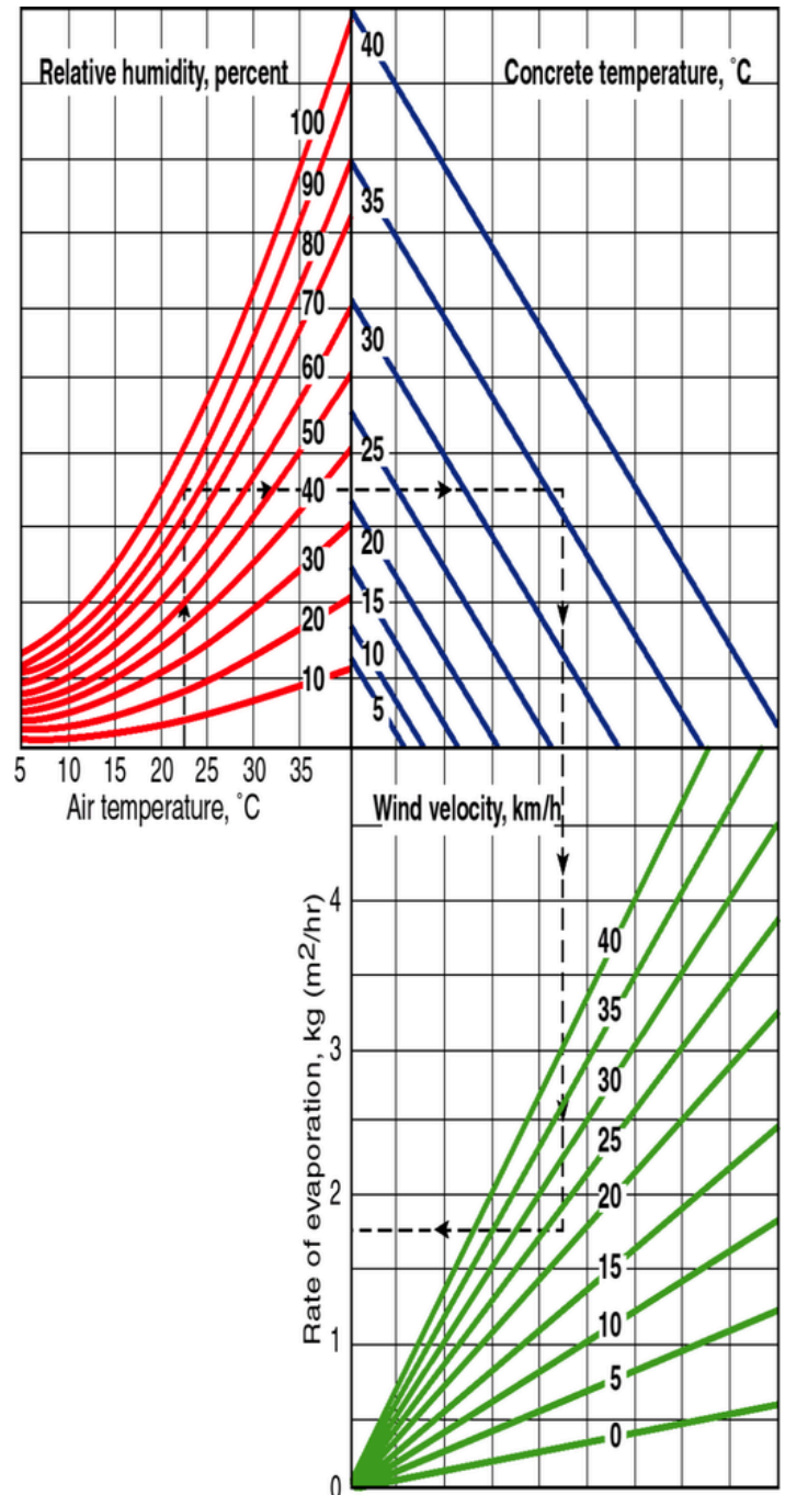
Effect of concrete and air temperatures, relative humidity, and wind velocity on rate of evaporation of surface moisture from concrete (Menzel, 1954).
